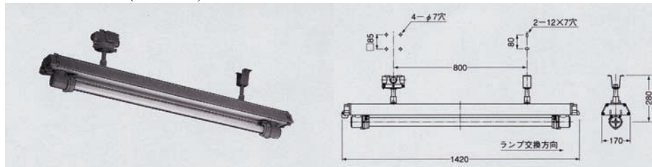
EXIF141225 (1 x 40W)
